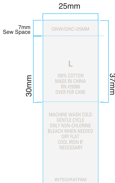
HG-1097 GNW/GNC-25MM
